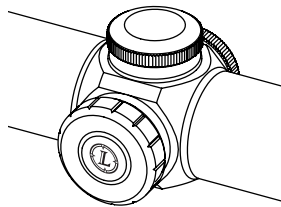
The Push Button control for the Leupold VX-R and VX-6 Illuminated Reticle is located on the adjustment turret.
