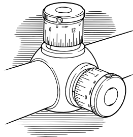
Target style adjustments for range and wind adjustments in the field.
