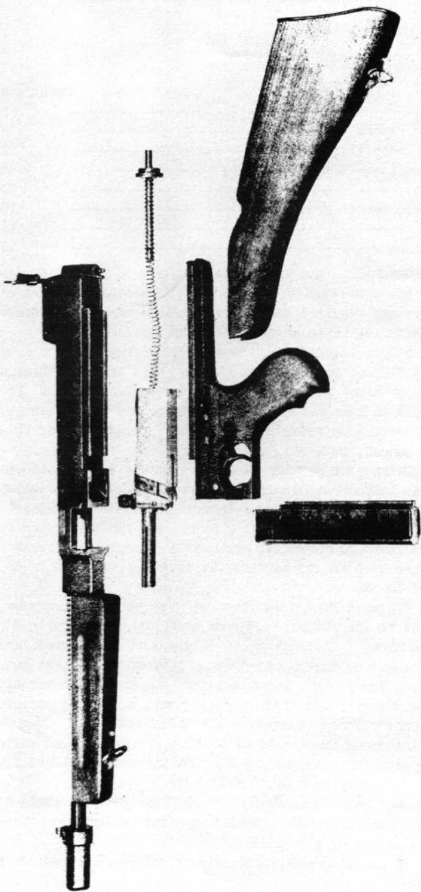
FIGURE 3 — THOMPSON SUBMACHINE GUN, CAL. .45, M1928A1 - GROUPS
