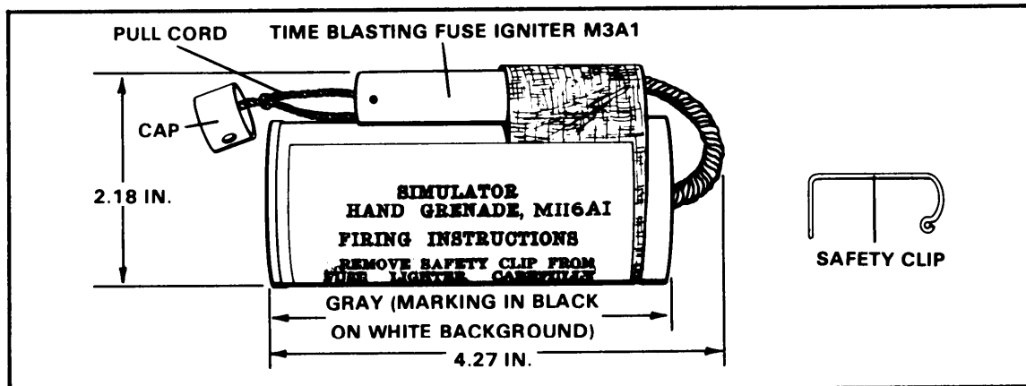
Figure 5-6. M116A1 simulator.
