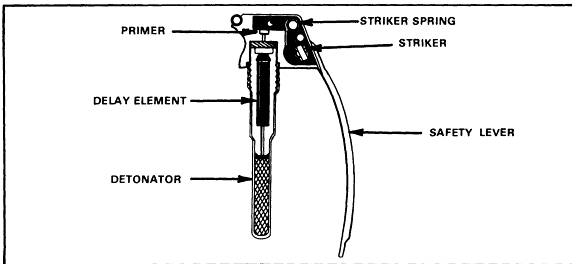
Figure 1-3. M204A2 fuze.
