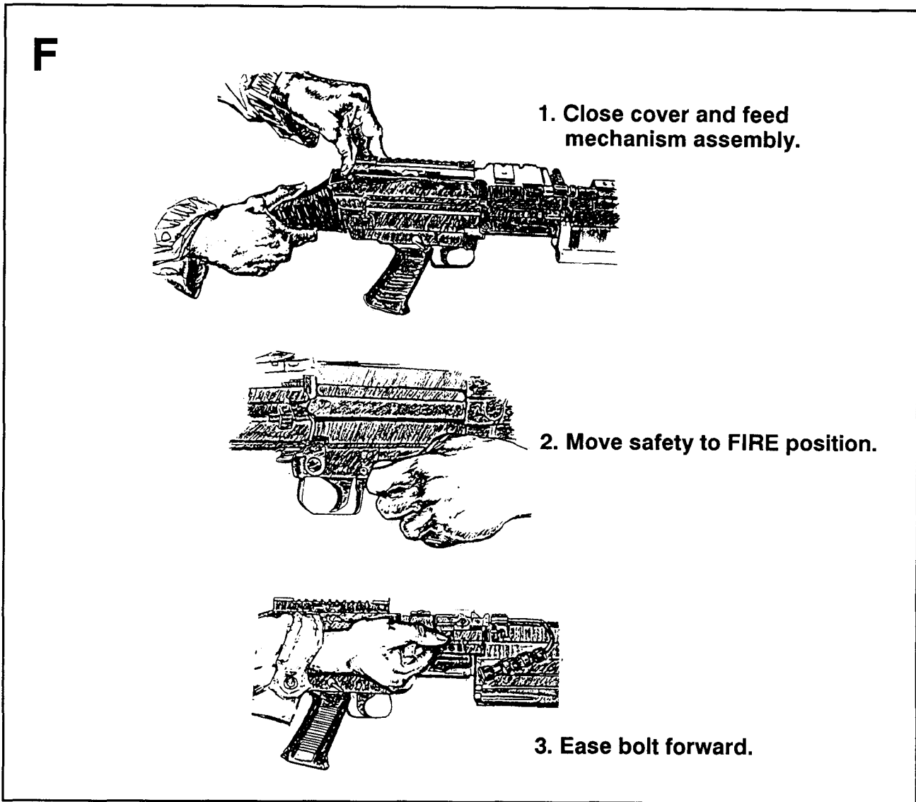
Figure 2-1. Clearing procedures (continued).
