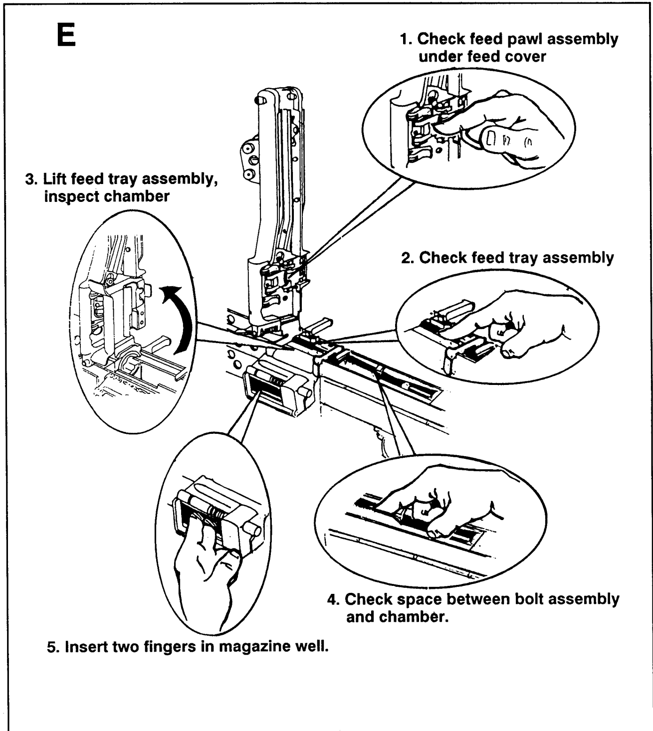
Figure 2-1. Clearing procedures (continued).
