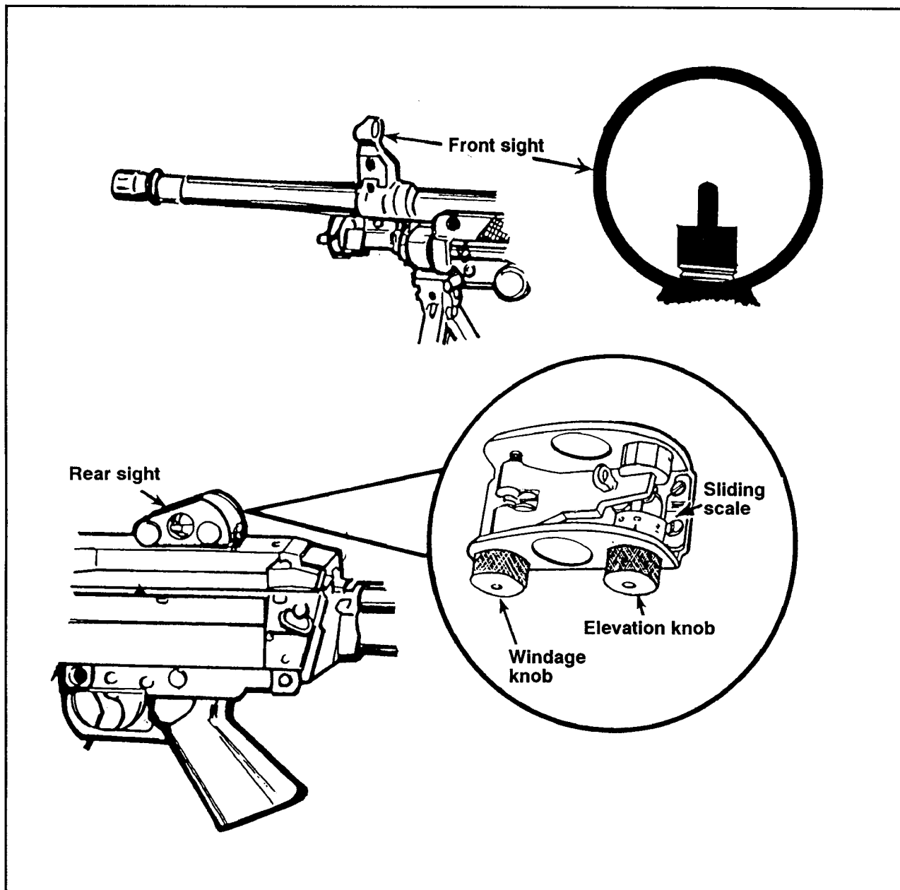
Figure 1-3. Sights.
